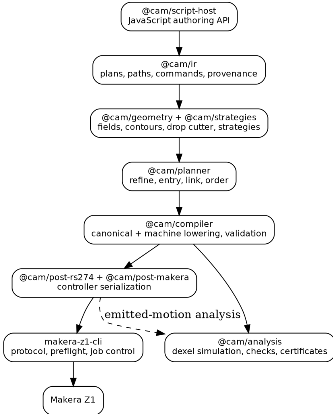
Figure 36.1: The reviewed Dropcut package architecture and controller boundary.
